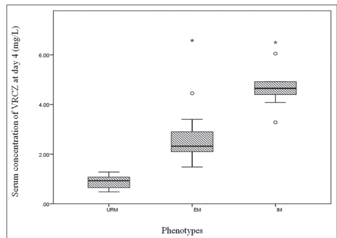
Figure 2: Comparison of serum concentrations of voriconazole in ultra-rapid, extensive, and intermediate metabolizer phenotypes. There was a significant difference in serum levels in different phenotypes ( P < 0.00001 )
